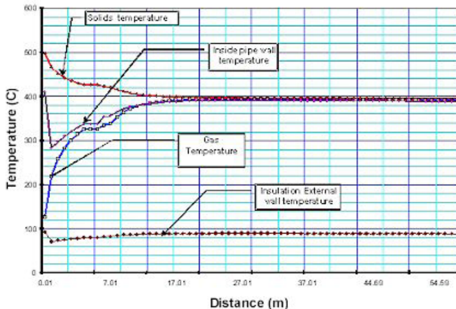
Figure 4: Temperatures as Measured from Inlet - Down the Pipeline
