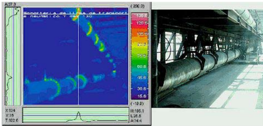
Figure 3: Thermograph of the double pneumatic conveying line on top of the melt shop. Bright spots correspond to location of pipeline supports.
