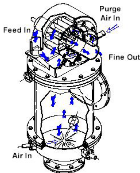
Figure 1. Dense Phase Mill
