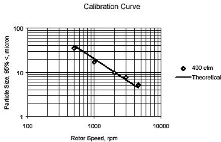
Figure 2. Theoretical vs. Actual Milling Size
